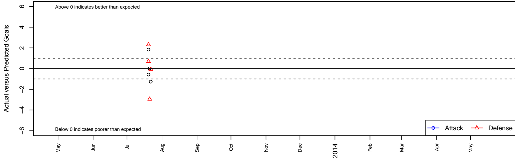
MSC Polaris 03 G02 Dots are actual minus expected GF (blue circles) and GA (red triangles). Blue line is smoothed change in attack strength. Red is smoothed change in defense strength.
